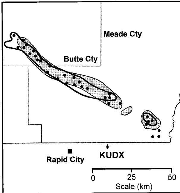
FIG. 6. Areal extent of the surface damage from the 5–6 July 1996 Butte–Meade storm. Reports of hail greater than 5 cm are indicated by filled circles; the region encapsulating reports of F1 or greater wind damage is indicated by the thick line. The shaded areas indicate storm-damaged areas apparent in the GOES-8 visible satellite imagery.
