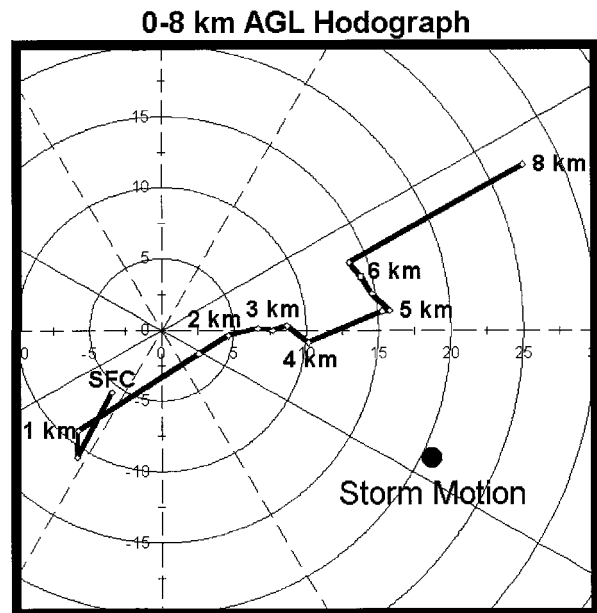
FIG. 4. Hodograph of the winds from the 0000 UTC Rapid City sounding, modified in the low levels with 0500 UTC surface data and KUDX radar VWP data. Horizontal and vertical axes are in meters per second. Numbers along the hodograph line are heights in kilometers AGL.
