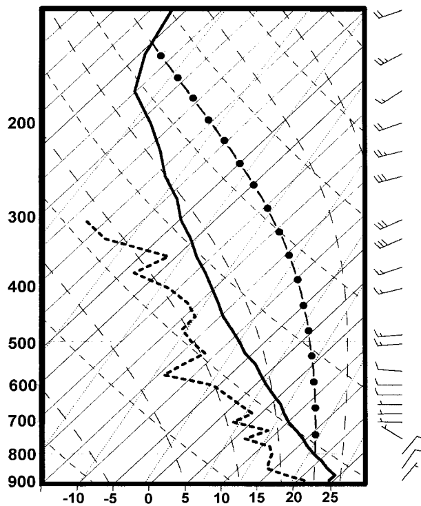
FIG. 3. Skew T - \log p diagram representing the temperature (solid line), moisture (dashed line), and wind profile over Rapid City at the time of the storm (0500 UTC 6 July). Horizontal axis is temperature ( ^{\circ}\text{C} ); vertical axis is pressure (mb). The wind is given along the right edge, with a full barb representing 10\text{ m s}^{-1} . The 0000 UTC Rapid City sounding was modified with (0500 UTC) surface data and VAD wind profile data from the KUDX radar for this figure.
