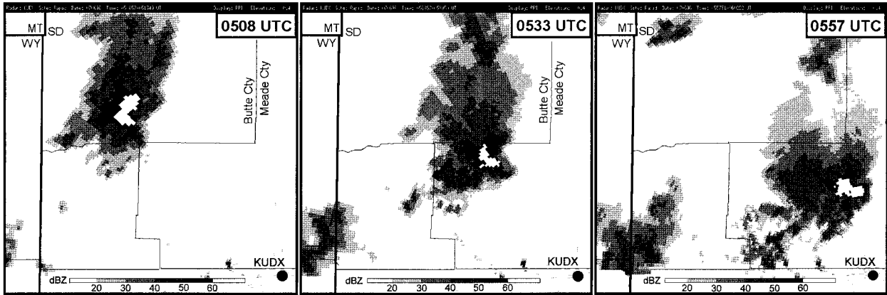
FIG. 5. Plots of the KUDX radar 0.5° reflectivity at 0508, 0533, and 0557 UTC. Reflectivity contoured every 10 dBZ, from 20 to 60 dBZ.
