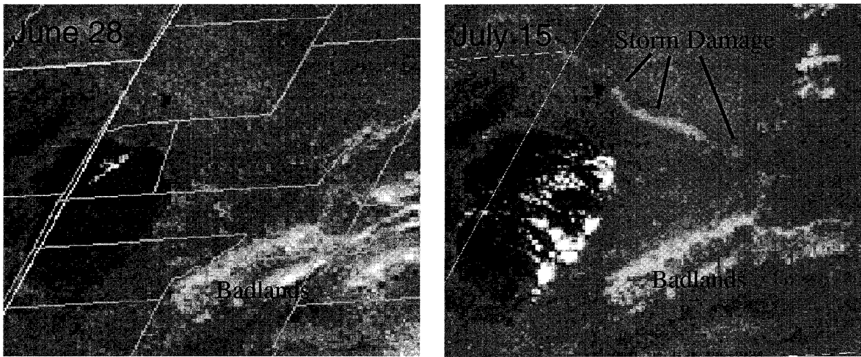
FIG. 1. GOES-8 visible satellite images taken before (left) and after (right) the 5–6 July 1996 Butte–Meade storm, illustrating the region of storm damage in western South Dakota.
