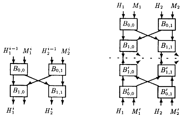
Fig. 2. The g_{2,1} compression function and the corresponding collision network
