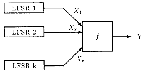
Fig. 1. Combining LFSRs
