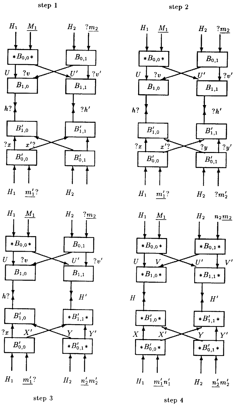
Fig. 3. Resolution of the collision network for g_{2,1}
